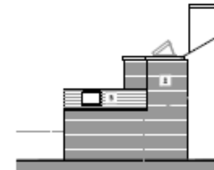
EAST ELEVATION (1:100)
