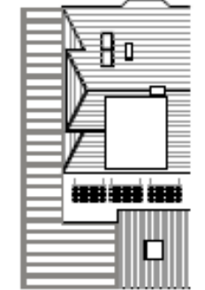
ROOF PLAN (1:100)
