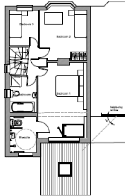
FIRST FLOOR PLAN (1:50)
